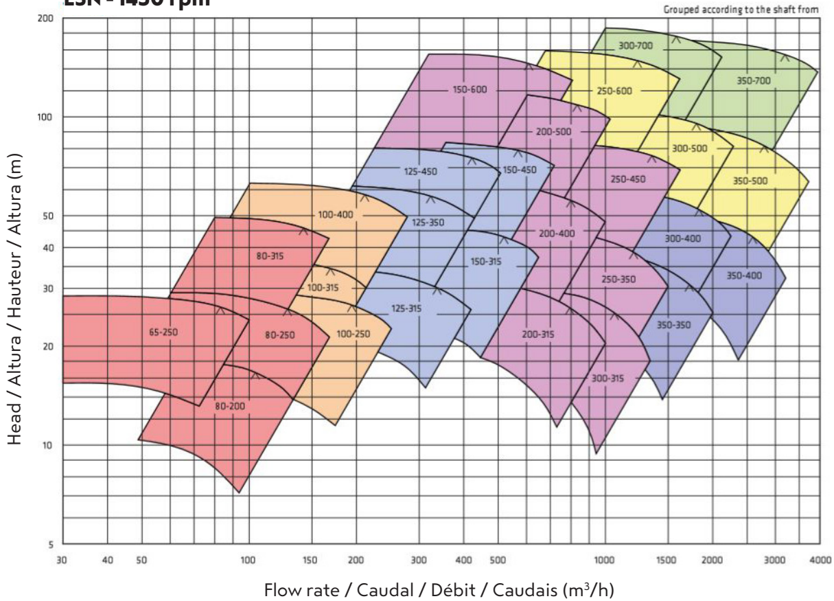
ESN - 1450 rpm
