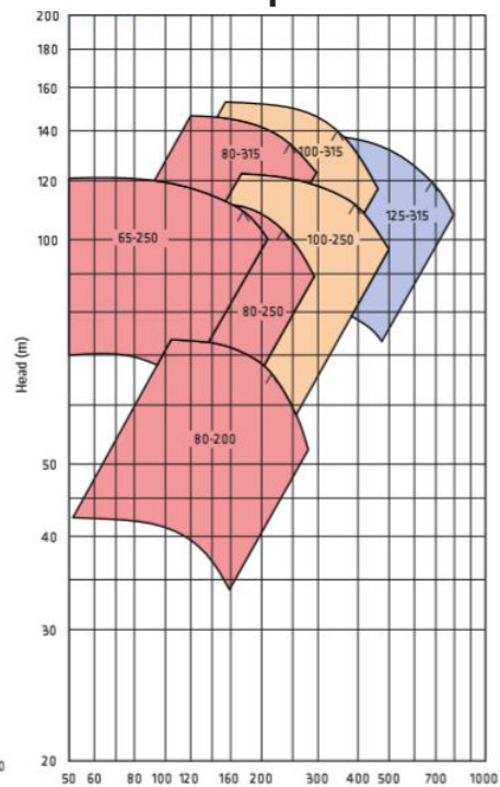
SCP - 2900 rpm
